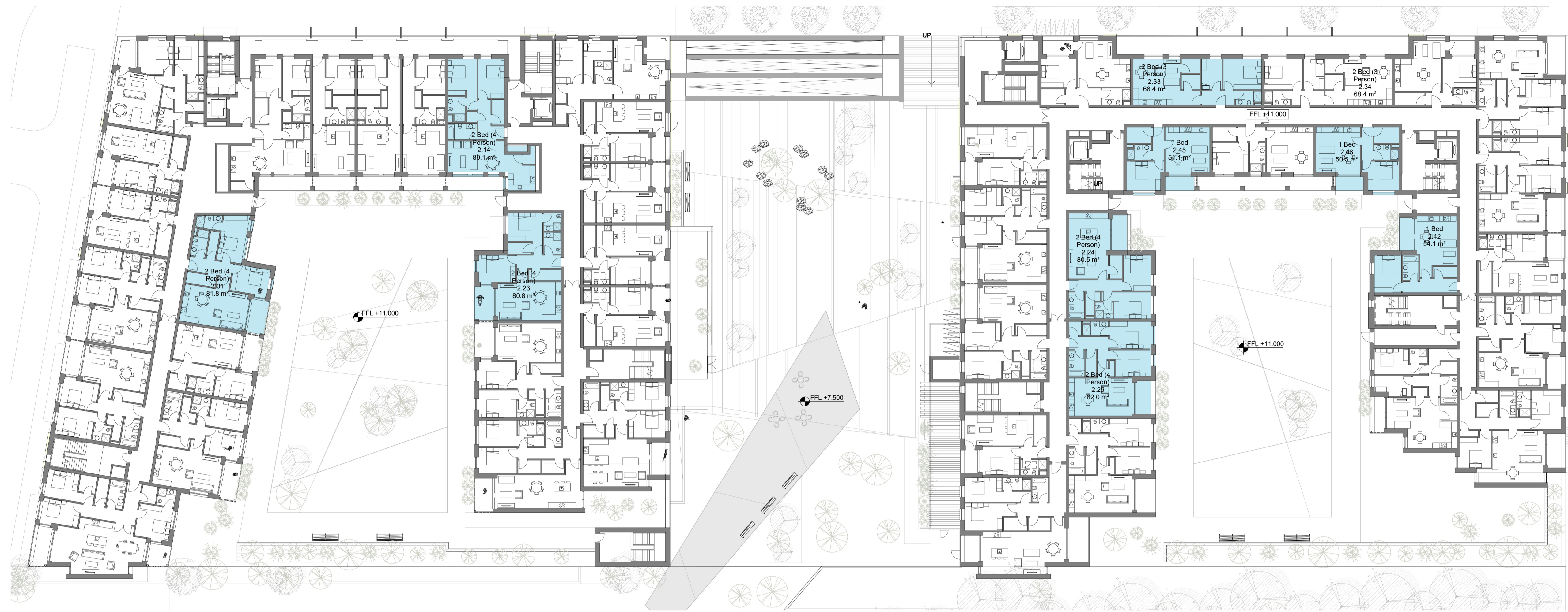
1 GA - LV02 - PART V ALLOCATION - 9 UNITS 1 : 250
